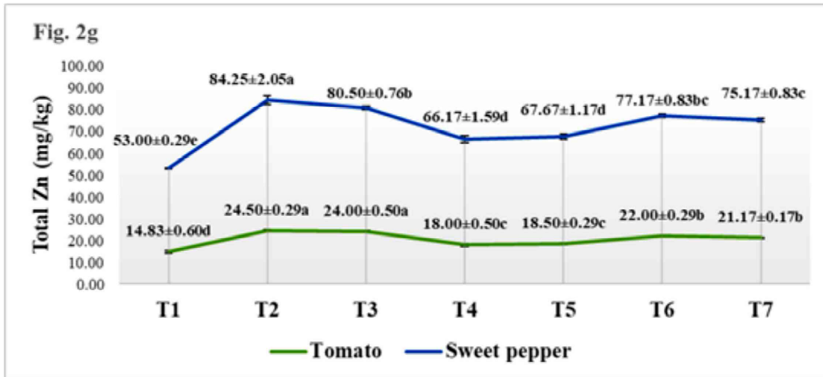
Fig. 2 : Effect of ZnO nanoparticles on nutrient content in tomato and sweet pepper
