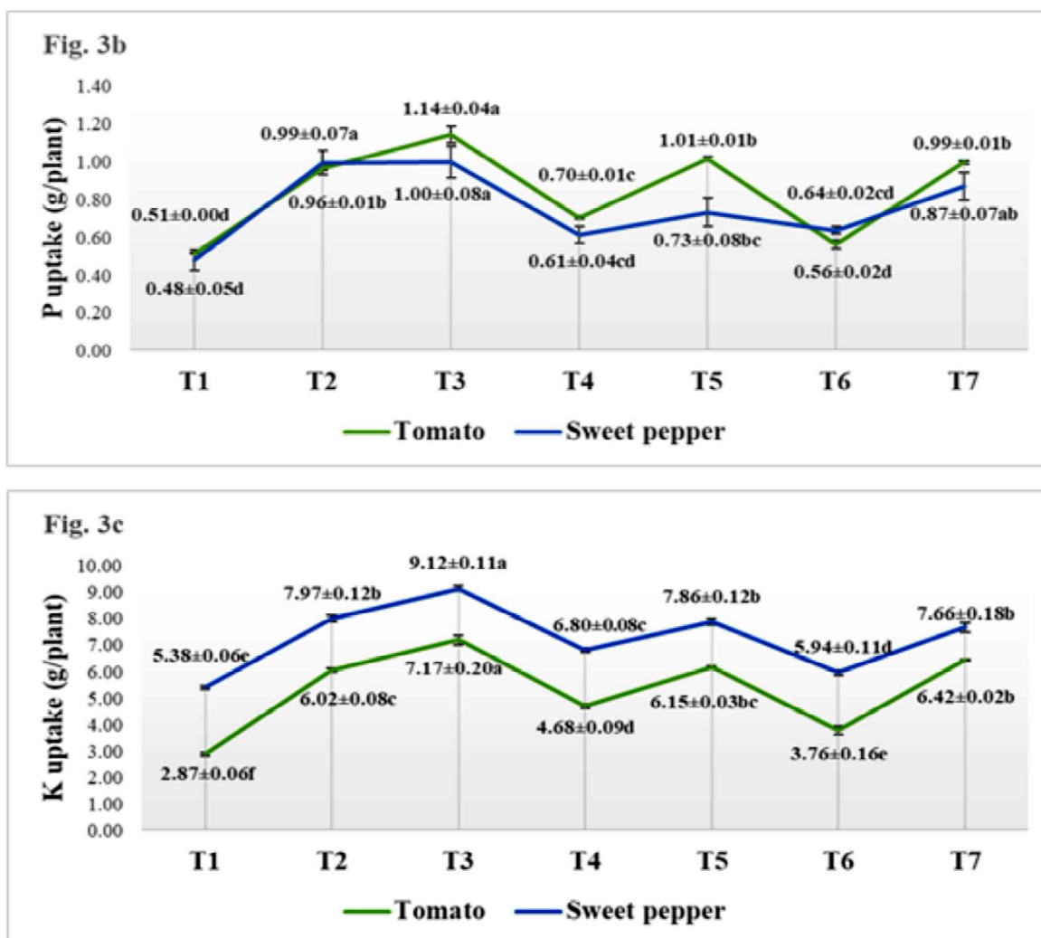
Fig. 3 : Effect of ZnO nanoparticles on nutrient uptake in tomato and sweet pepper
