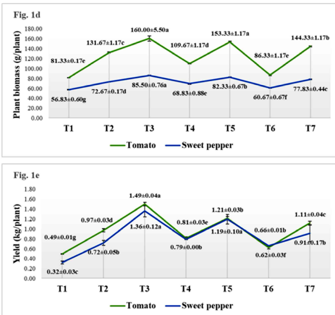
Fig. 1 : Effect of ZnO nanoparticles on growth parameters of tomato and sweet pepper
